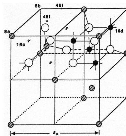
Figure 1. Two quadrants of the cubic \text{A[B}_2\text{]O}_4 spinel structure: A cations at 8a (hatched circles), B cations at 16d (solid circles), and oxygen at 48f (white circles).
